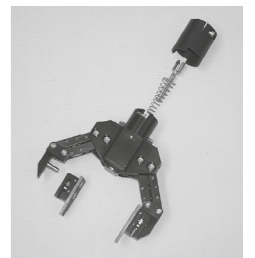
Tongs PMC 97 with disconnectable grippers
